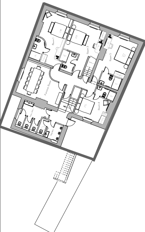
2 First Floor: Proposed Scale 1:100
