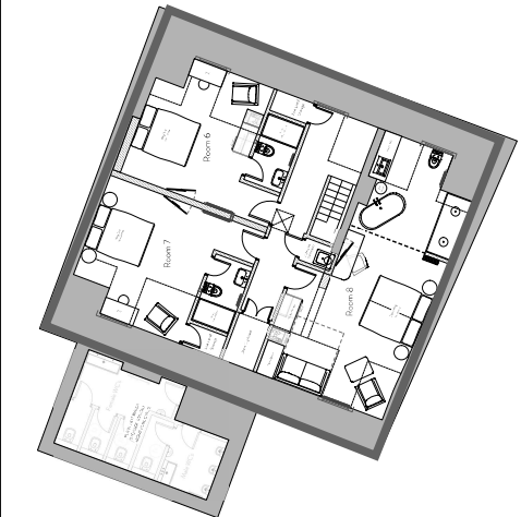
3 Second Floor: Proposed Scale 1:100
